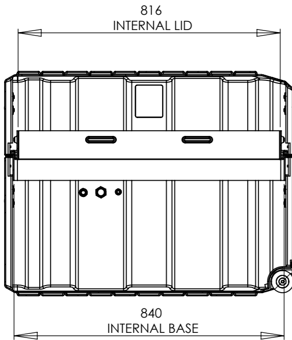
SECTION Y-Y SCALE 1 : 12
