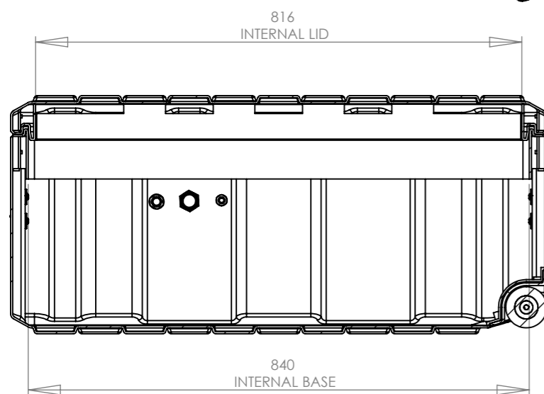
SECTION Y-Y SCALE 1 : 9
