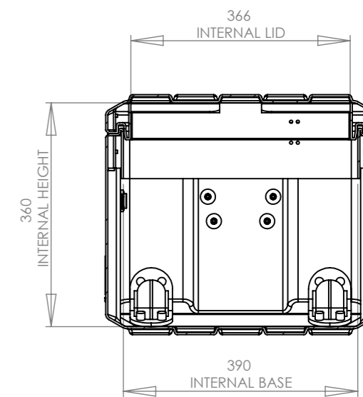
SECTION Z-Z SCALE 1 : 9
