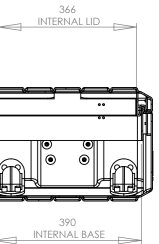
SECTION Z-Z
