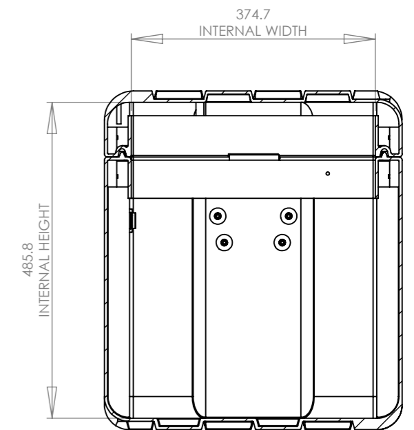
SECTION Z-Z
