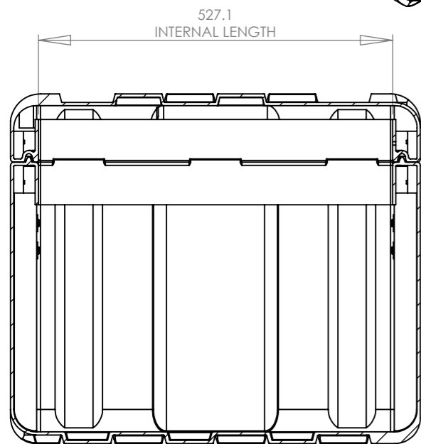
SECTION Y-Y
