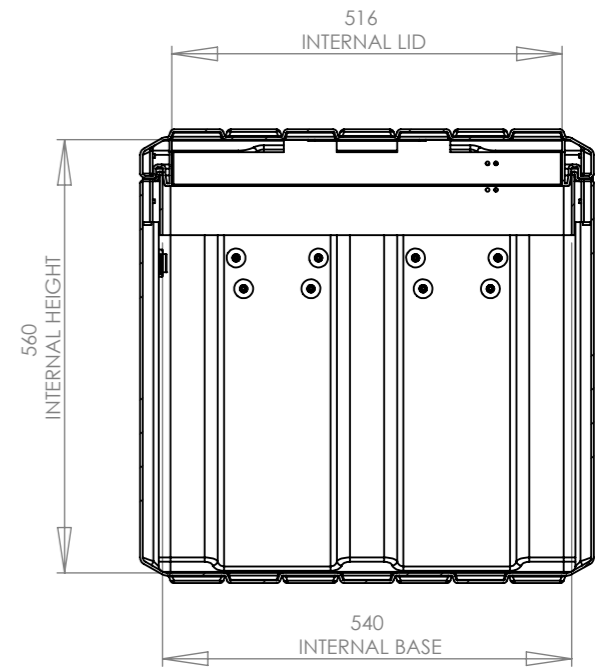
SECTION Z-Z
